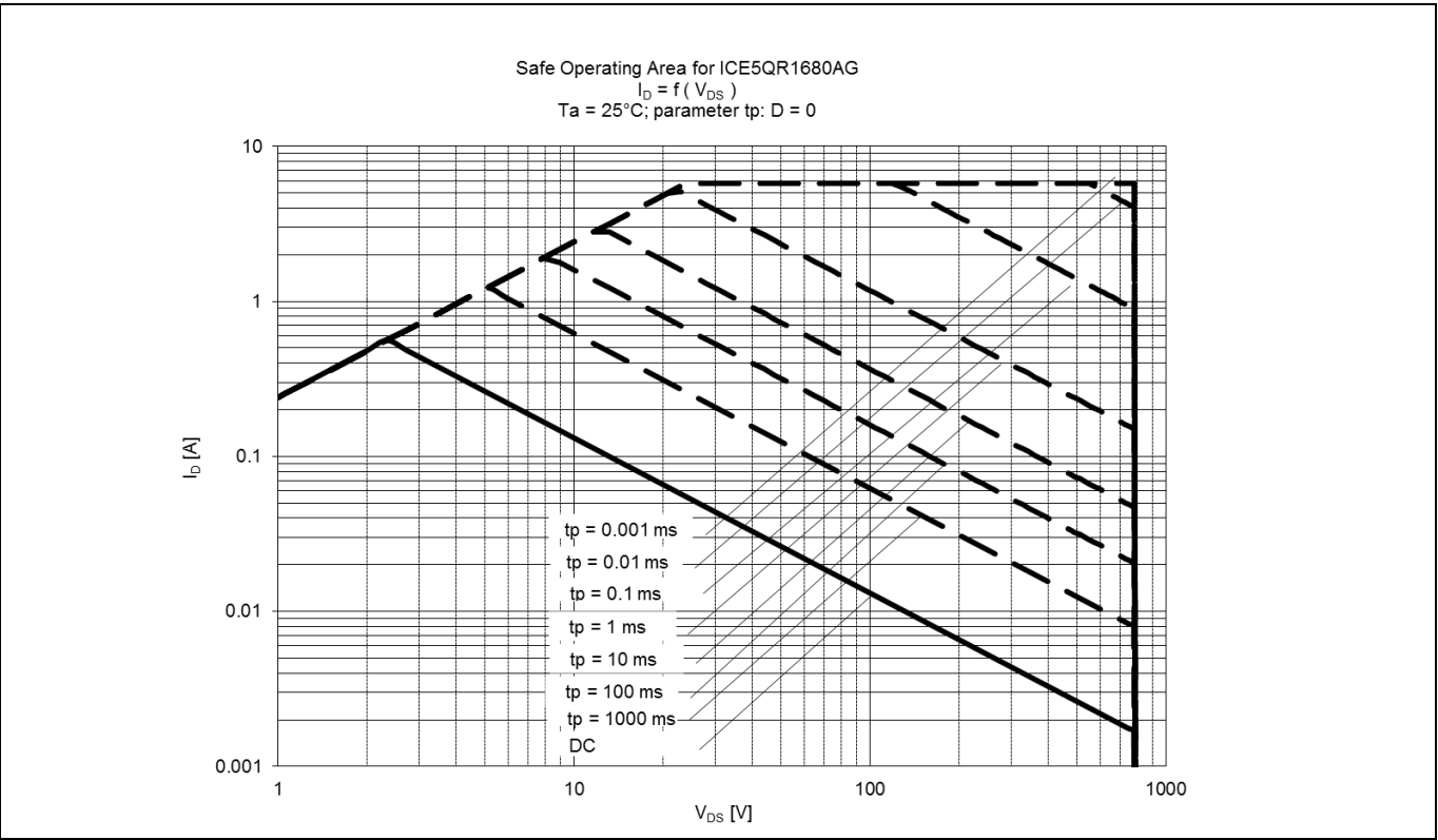
Figure 21 Safe Operating Area (SOA) curve for ICE5QR1680AG
