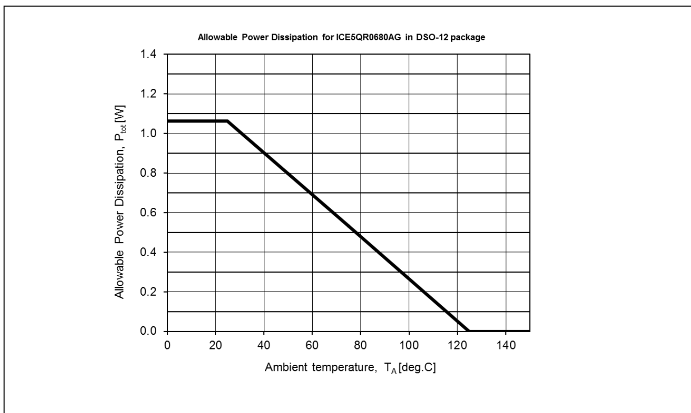
Figure 31 Power dissipation of ICE5QR0680AG, DSO-12 package; P_{tot}=f(T_a) , (Maximum ratings as given in section 4.1 must not be exceeded)
