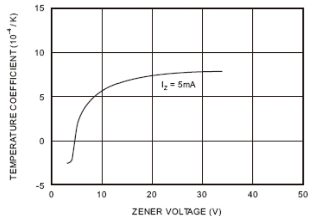
FIG. 4-TEMPERATURE COEFFICIENT OF V_Z VS. Z-VOLTAGE
