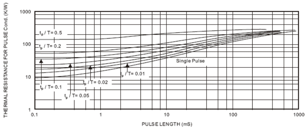
FIG. 10-THERMAL RESPONSE
