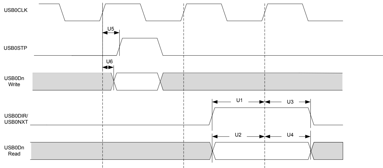
Figure 30-41. ULPI Interface Timing Diagram
