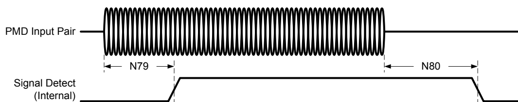
Figure 30-40. 100Base-TX Signal Detect Timing
