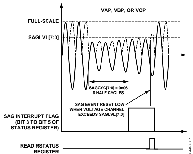
Figure 57. ADE7758 SAG Detection
