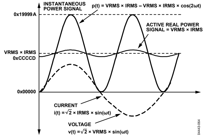
Figure 65. Active Power Calculation
