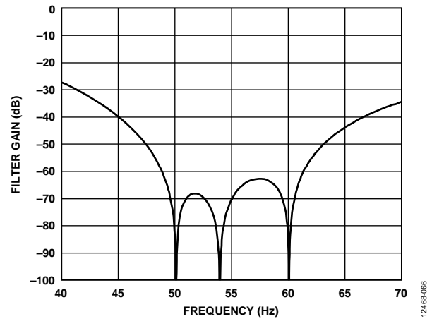
Figure 66. 25 SPS ODR, 40 ms Settling Time
