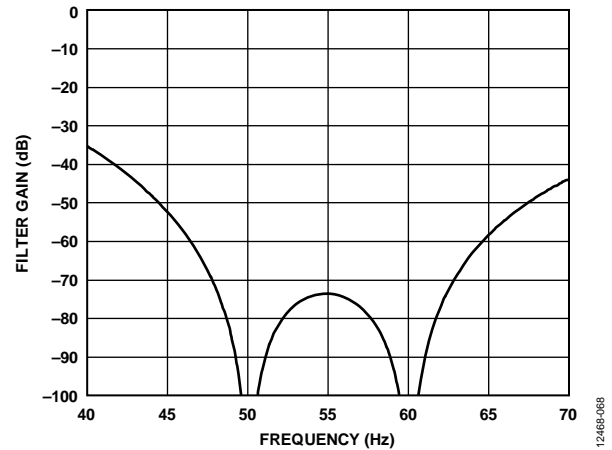
Figure 67. 20 SPS ODR, 50 ms Settling Time
