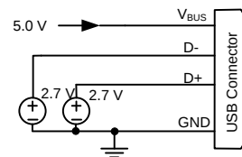
Figure 11. Divider 3 DCP
