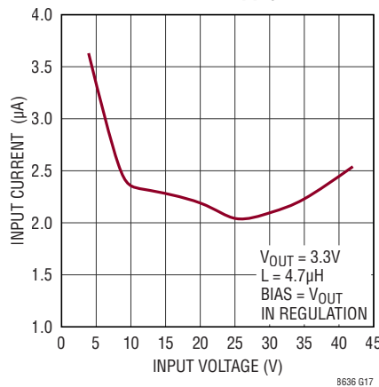
LT8636 No-Load Supply Current
