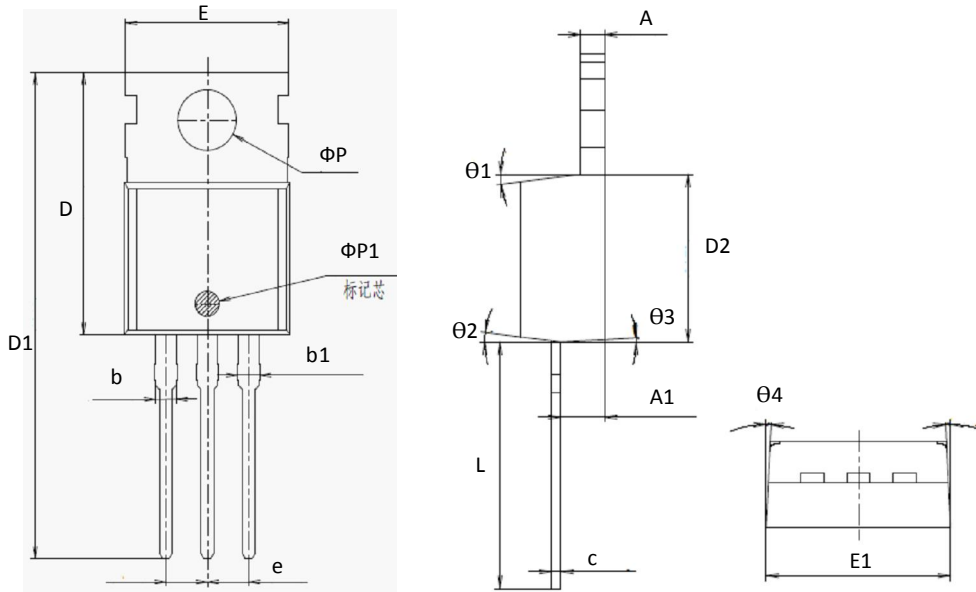
TO220 PACKAGE OUTLINE DIMENSION_GN
