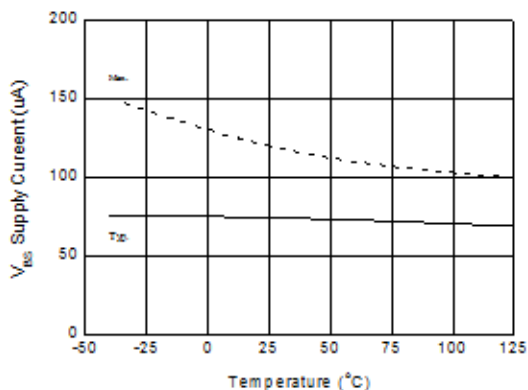
Figure 43. V_{BS} Supply Current vs. Temperature ( V_{BS}=15\text{ V} )
