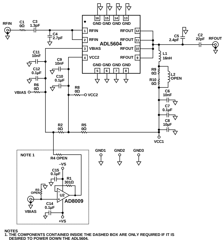
Figure 35. Basic Connections
