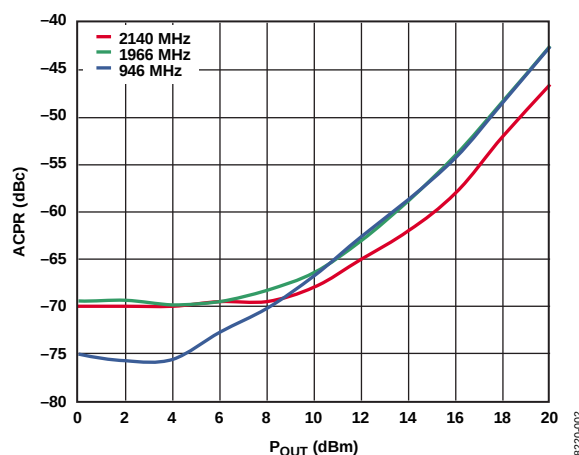
Figure 2. ACPR vs. Output Power, 3GPP 3.5 TM1-64
