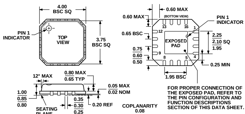
Figure 47. 16-Lead Lead Frame Chip Scale Package [LFCSP_VQ] 4 mm × 4 mm Body, Very Thin Quad (CP-16-4)
