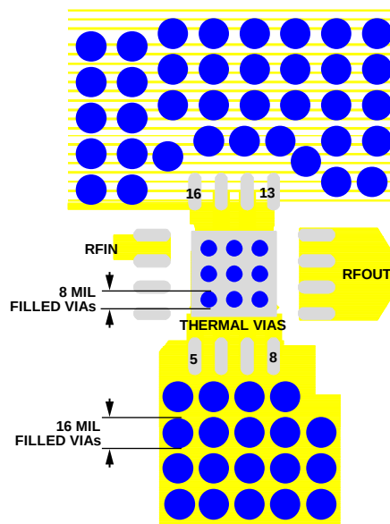
Figure 42. Recommended Land Pattern
