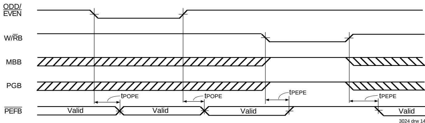
Figure 11. ODD/ \overline{\text{EVEN}} , W/RB, MBB, and PGB to \overline{\text{PEFB}} Timing
