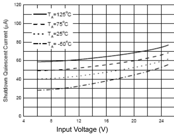
Figure 5. Shutdown Quiescent Current vs. Input Voltage
