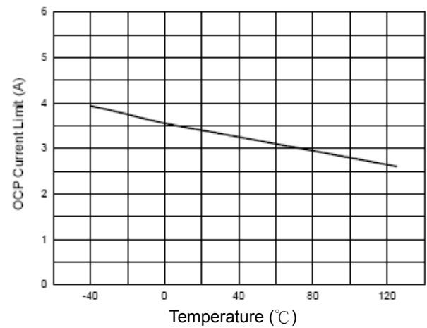
Figure 6. OCP Current Limit vs. Temperature
