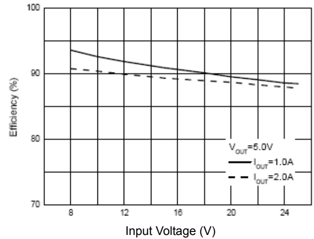
Figure 4. Efficiency vs. Input Voltage
