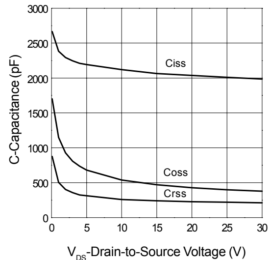
Capacitance Characteristics
