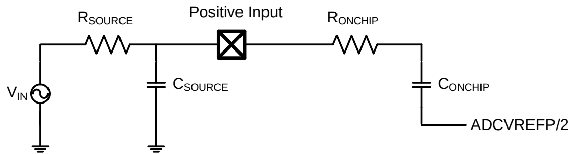
Figure 32-7. ADC Input
