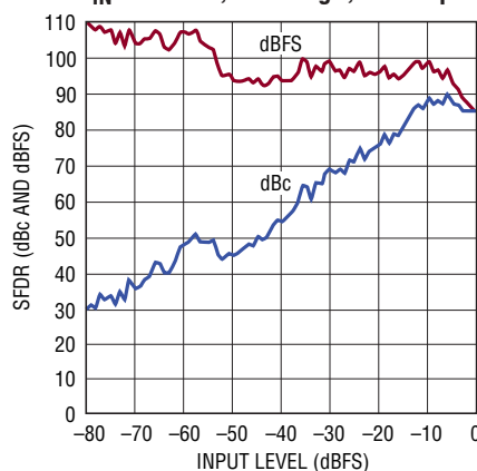
LTC2267-14: SFDR vs Input Level, f_{IN} = 70\text{MHz} , 2\text{V} Range, 105\text{Mps}
