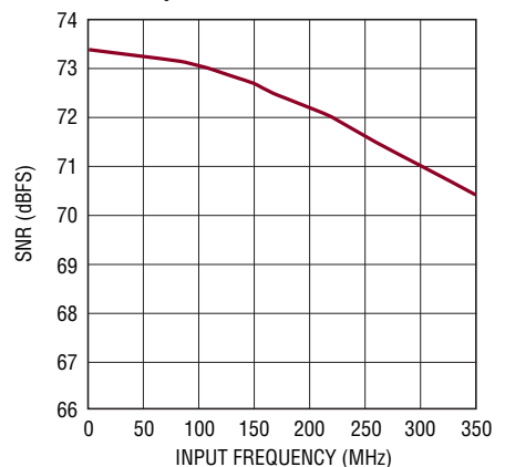
LTC2267-14: SNR vs Input Frequency, -1\text{dB} , 2\text{V} Range, 105\text{Mps}
