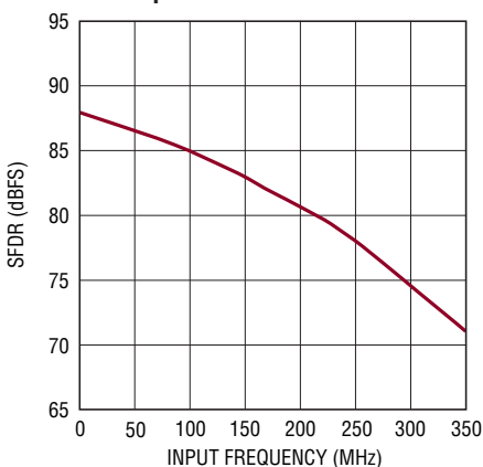
LTC2267-14: SFDR vs Input Frequency, -1\text{dB} , 2\text{V} Range, 105\text{Mps}
