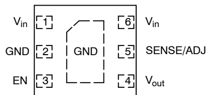
NCV8606, DFN6 3x3.3mm (Top View)
