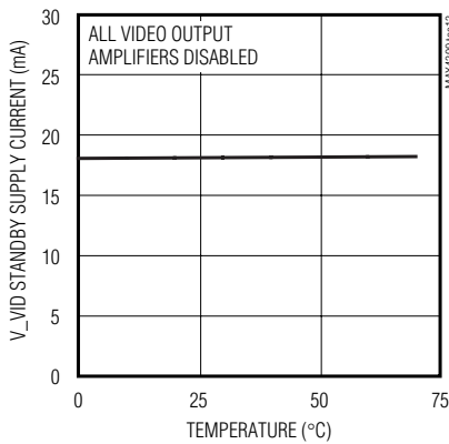
V_VID STANDBY QUIESCENT SUPPLY CURRENT vs. TEMPERATURE
