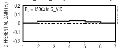
RF_CVBS_OUT (WITH TRAP FILTER)
