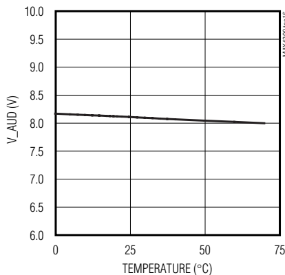
V_AUD vs. TEMPERATURE
