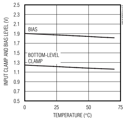
INPUT CLAMP AND BIAS LEVEL vs. TEMPERATURE
