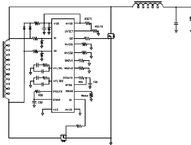
Fig. 1 Typical application circuit when supply V_{out} < 5.0 \text{ V}_{DC}
