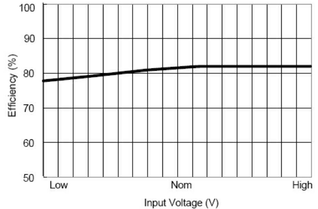
Efficiency vs Input Voltage ( Dual Output )
