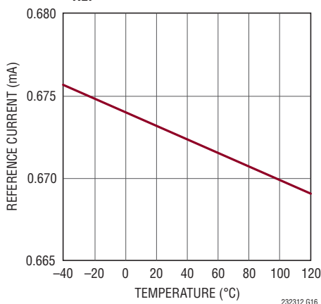
Reference Current vs Temperature, V_{REF} = 4.096\text{V}
