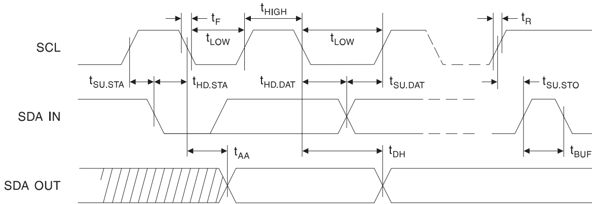
Figure 4. Bus Timing
