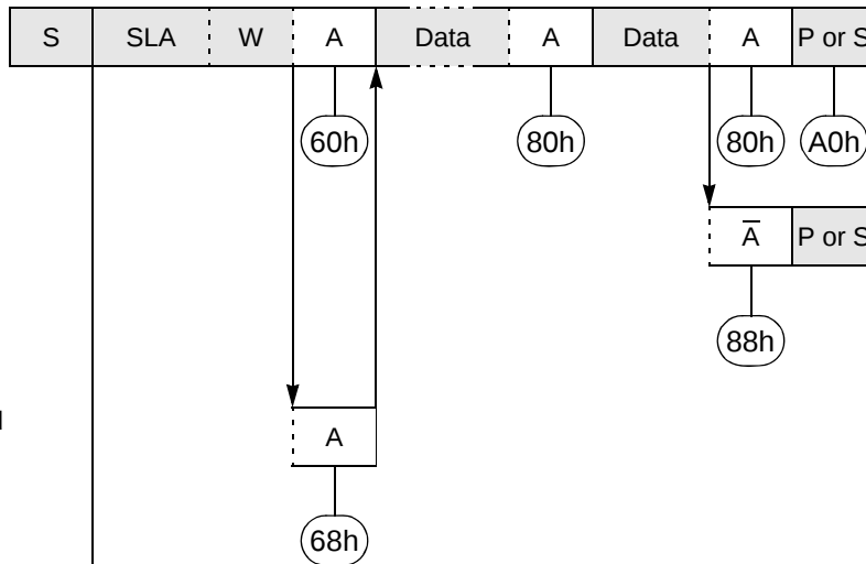
Figure 19-5. Format and States in the Slave Receiver Mode
