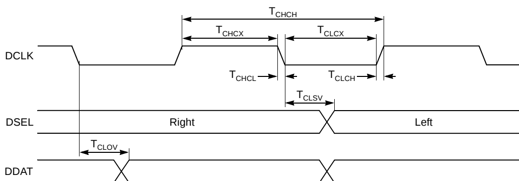
Figure 22-19. Audio Interface Waveforms
