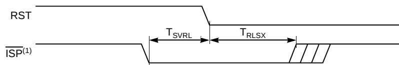
Figure 22-22. FLASH Memory - ISP Waveforms
