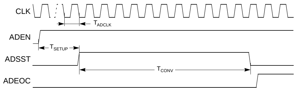
Figure 20-2. Timing Diagram
