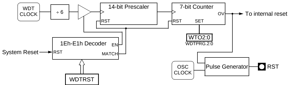
Figure 11-1. WDT Block Diagram
