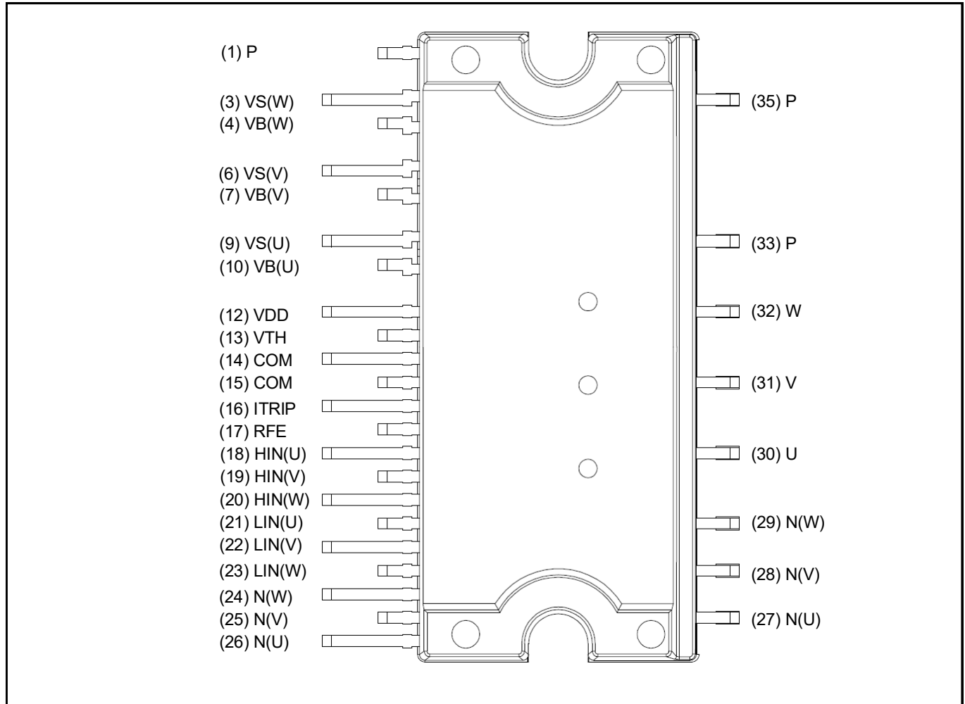
Figure 2 Pin configuration
