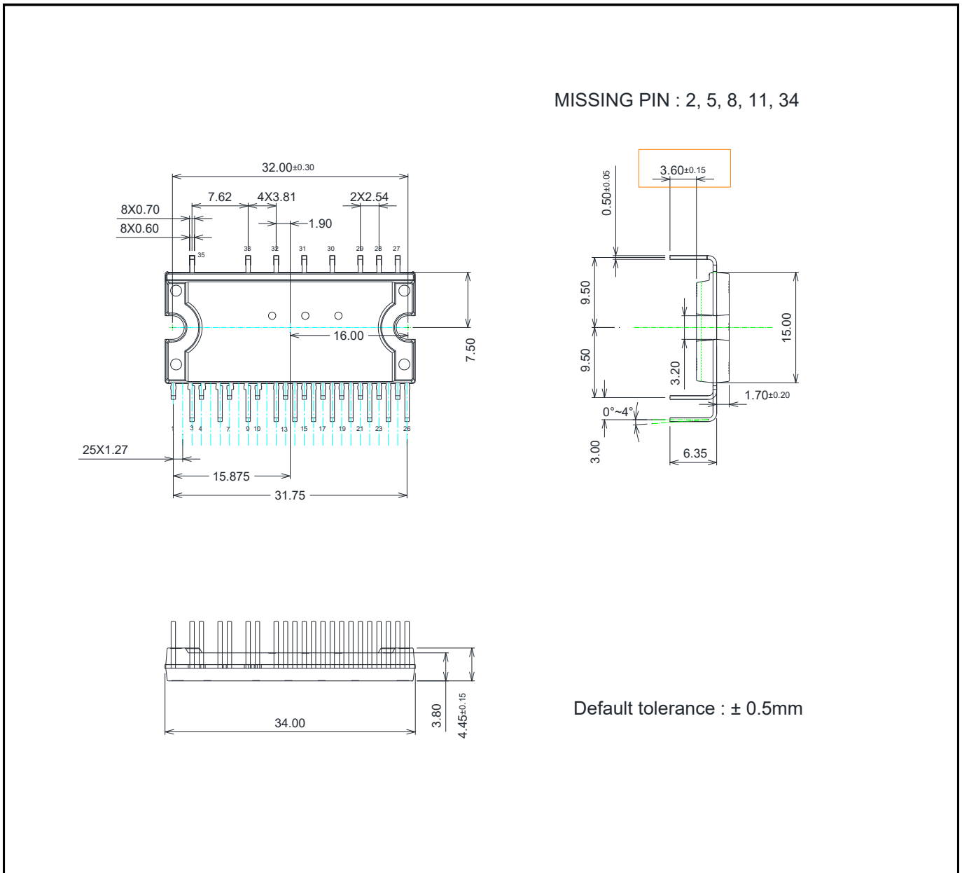
Figure 20 IM393-X6E3
