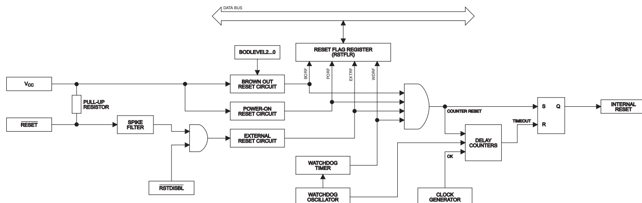
Figure 8-1. Reset Logic
