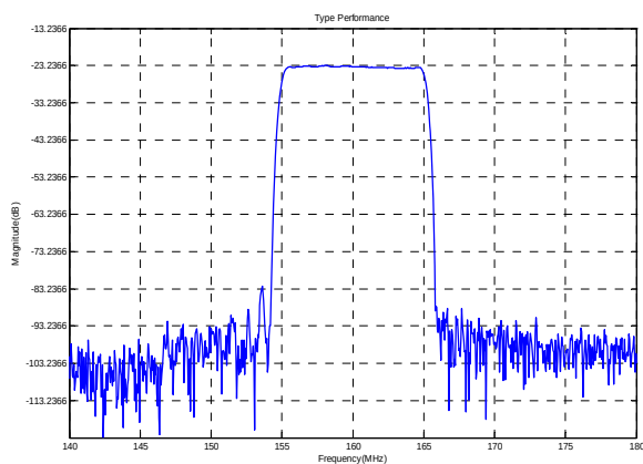
Frequency Respond
