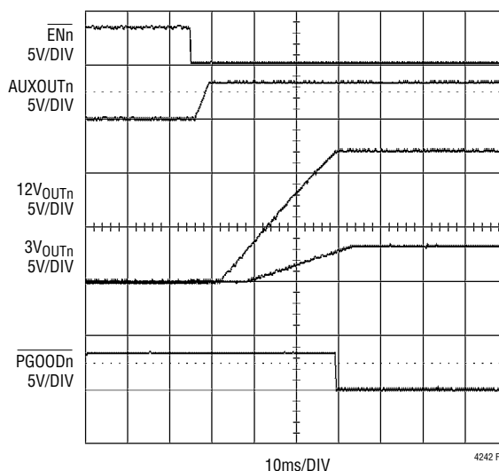
Figure 4. Normal Power-Up Sequence
