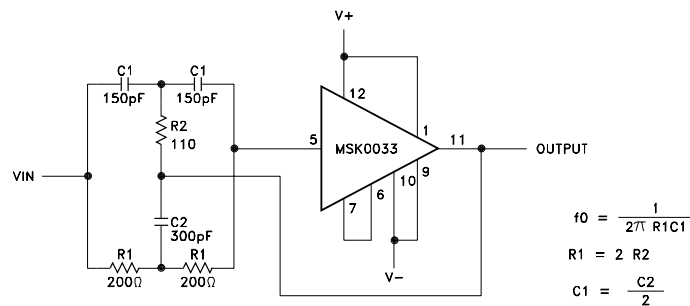
4.5MHz NOTCH FILTER
