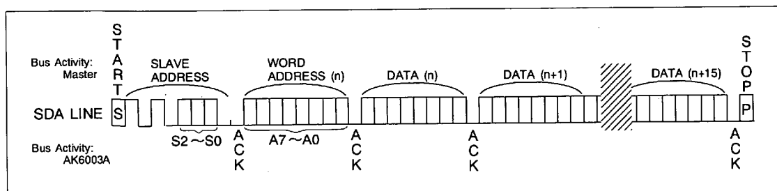
PAGE WRITE
