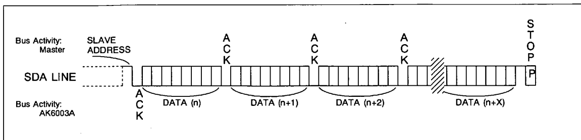
SEQUENTIAL READ
