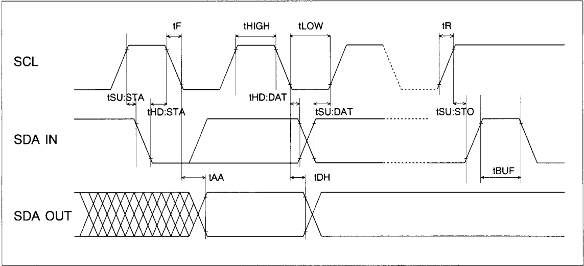
BUS TIMING
