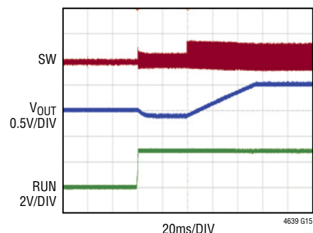
Start-Up Pre-Biased Load
