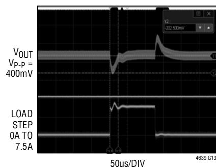
7V to 5V with 7.5A/μs Load Step, C_{PWR} = 5V
