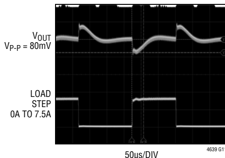
5V to 1.8V with 7.5A/μs Load Step, C_{PWR} = 5V
