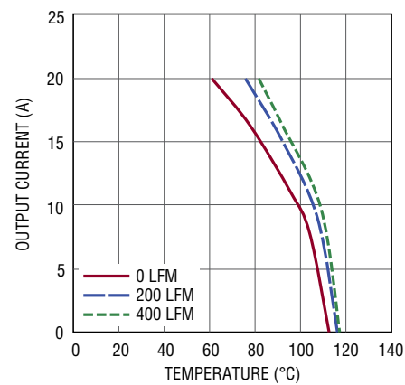
Figure 18. 7V IN to 2.5V OUT with Heat Sink
