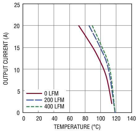
Figure 14. 7V IN to 1.0V OUT with Heat Sink
