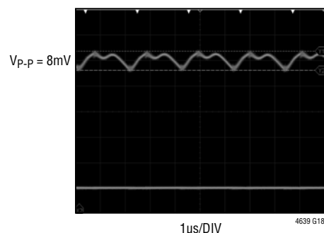
Output Ripple Noise
