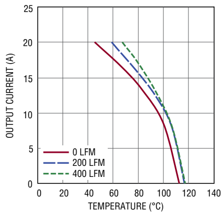
Figure 19. 7V IN to 5V OUT No Heat Sink, EXTV CC = 5V, C PWR = 7V
