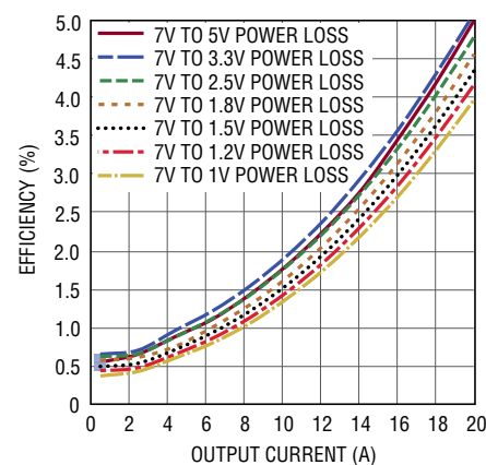
Figure 10. 7V Input Power Loss Curves
