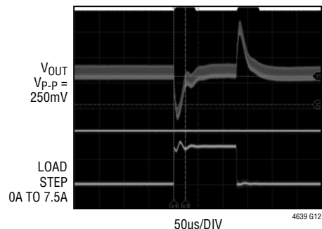
5V to 3.3V with 7.5A/μs Load Step, C_{PWR} = 5V
