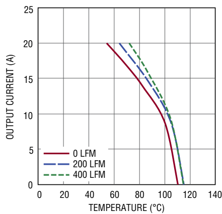
Figure 17. 7V IN to 2.5V OUT No Heat Sink
