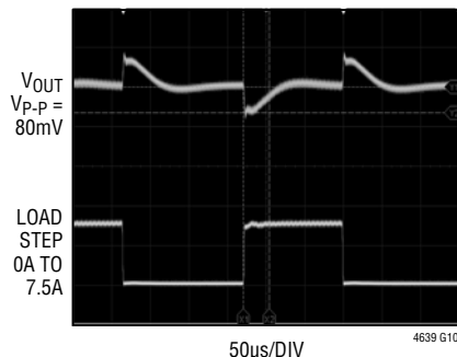
3.3V to 1.5V with 7.5A/μs Load Step, C_{PWR} = 5V
