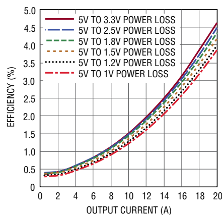
Figure 9. 5V Input Power Loss Curves
