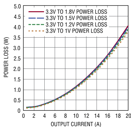
Figure 8. 3.3V Input Power Loss Curves
