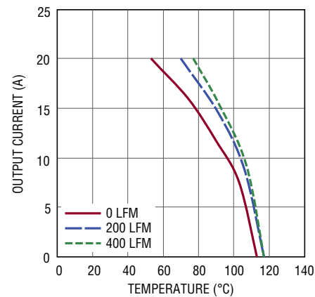
Figure 20. 7V IN to 5V OUT with Heat Sink, EXTV CC = 5V, C PWR = 7V
