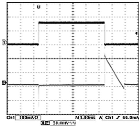
Load Transient 3.6V_{IN} , 2.5V_{OUT} , 0 – 150 mA load
