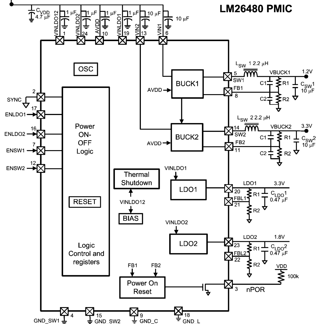
FIGURE 1. Application Circuit
