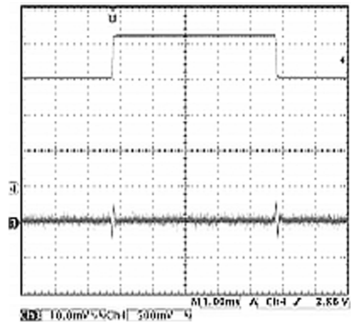
Line Transient (LDO2) 3.6 - 4.2V_{IN} , 1.8V_{OUT} , 150 mA load
