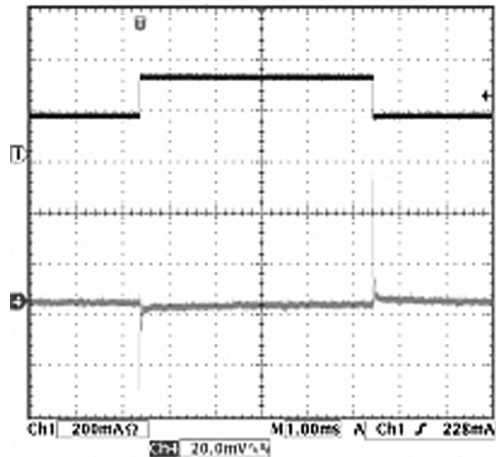
Load Transient 3.6V_{IN} , 2.5V_{OUT} , 150–300 mA load
