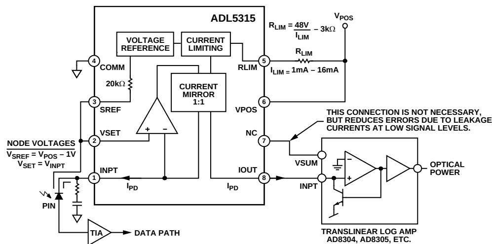
Figure 22. Typical Application Using the ADL5315
