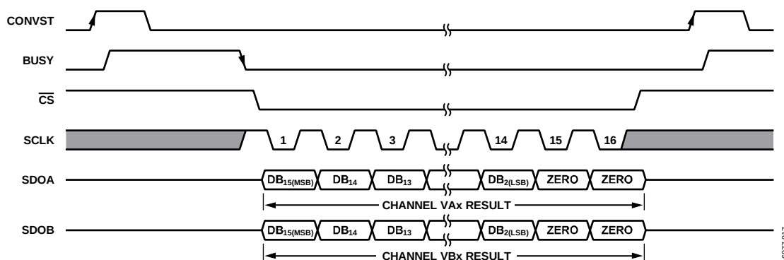
Figure 58. Serial Interface, 2-Wire Mode Reading Conversion Result
