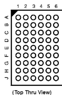
Pin Assignment for FBGA
