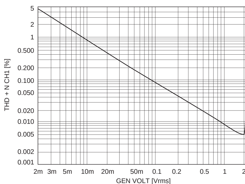
Graph 1. ADC Characteristics
