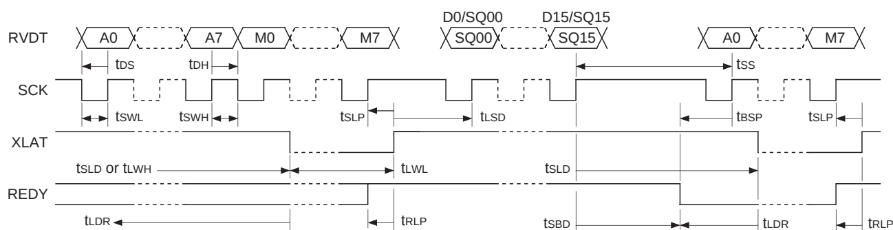
Fig. 5-2. Write Timing
