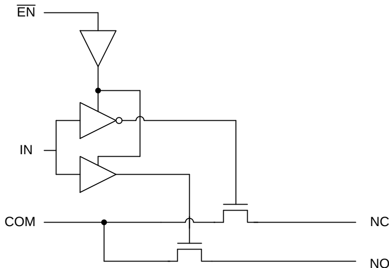
Block Diagram
