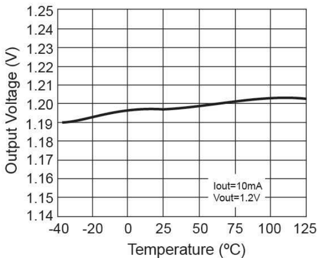
Figure 5. Output Voltage vs. Temperature
