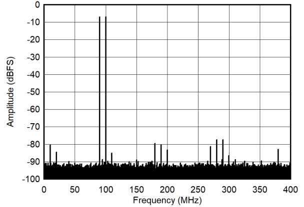
Figure 7-50. Single Tone FFT at 95 MHz
