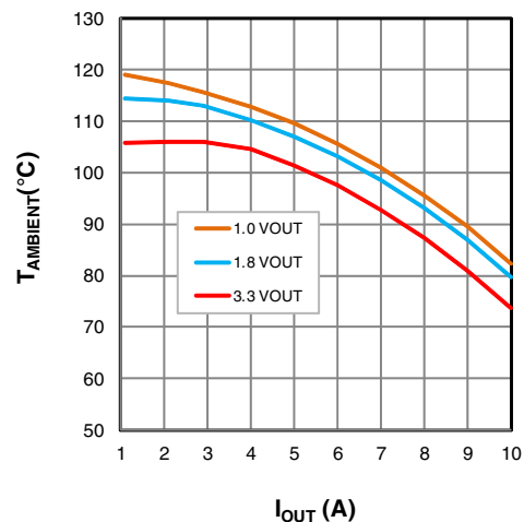
Figure 22: Maximum T_{\text{AMBIENT}} vs I_{\text{OUT}} , V_{\text{IN}}=12\text{V}
