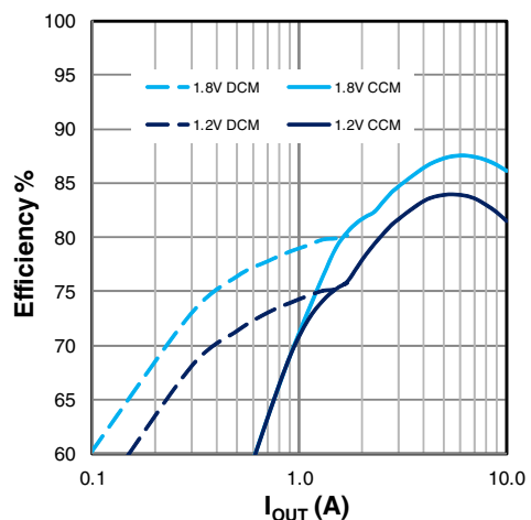
Figure 23: Efficiency, V_{\text{IN}}=19.6\text{V}
