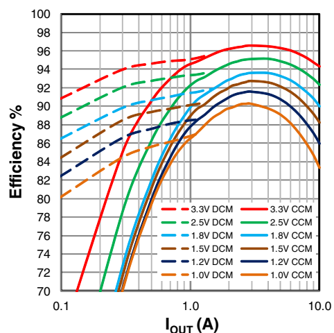
Figure 19: Efficiency, V_{\text{IN}}=5\text{V}
