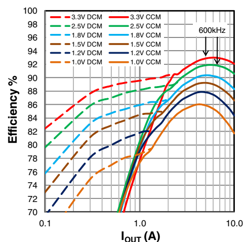
Figure 21: Efficiency, V_{\text{IN}}=12\text{V}
