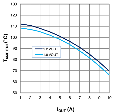
Figure 24: Maximum T_{\text{AMBIENT}} vs I_{\text{OUT}} , V_{\text{IN}}=19.6\text{V}
