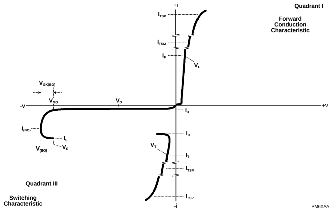
Figure 2. VOLTAGE-CURRENT CHARACTERISTIC
