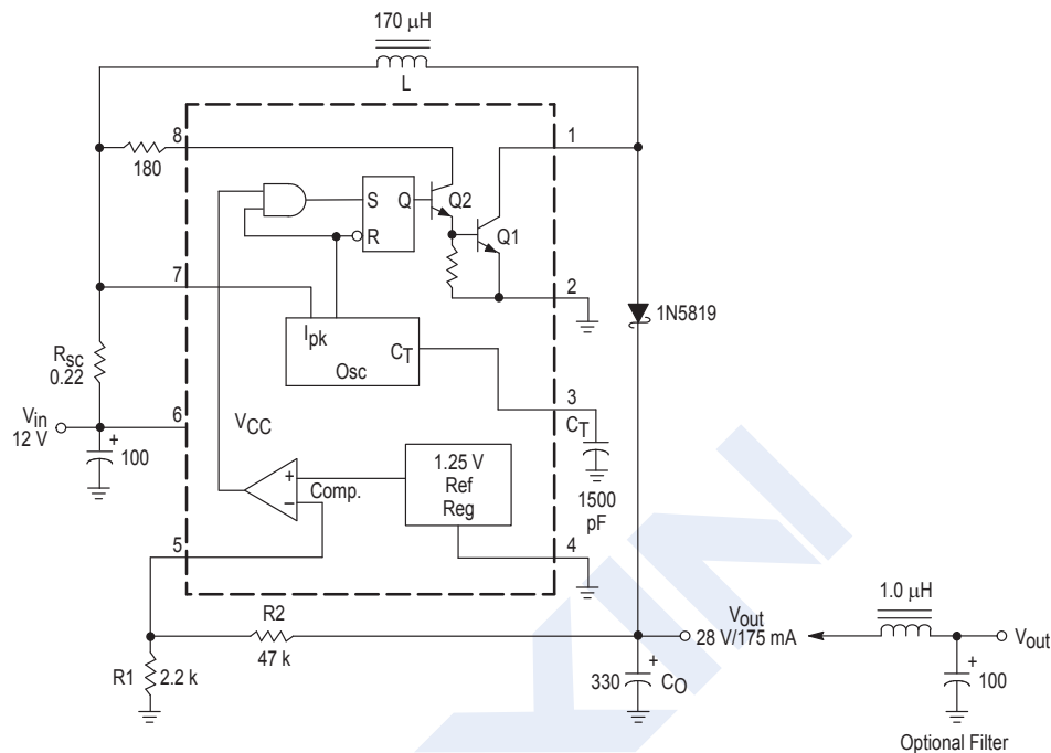
Figure 7. Step-Up Converter
