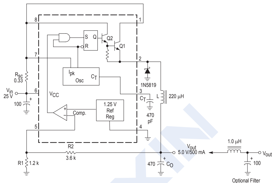
Figure 9. Step-Down Converter
