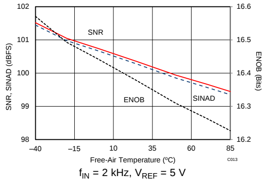
Figure 19. Noise Performance vs Temperature
