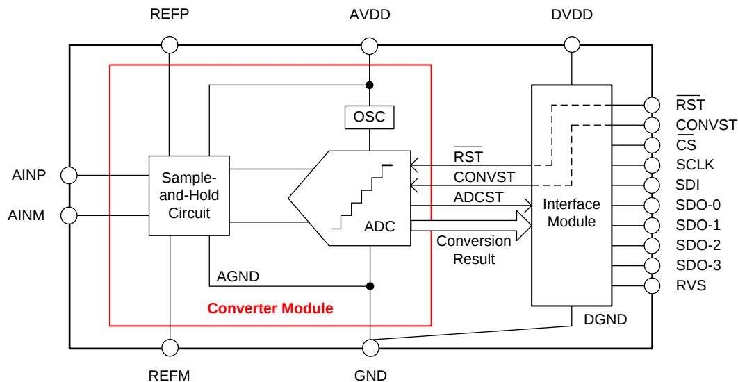
Figure 37. Converter Module
