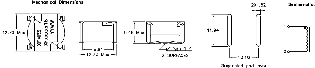
Mechanical Dimensions:
