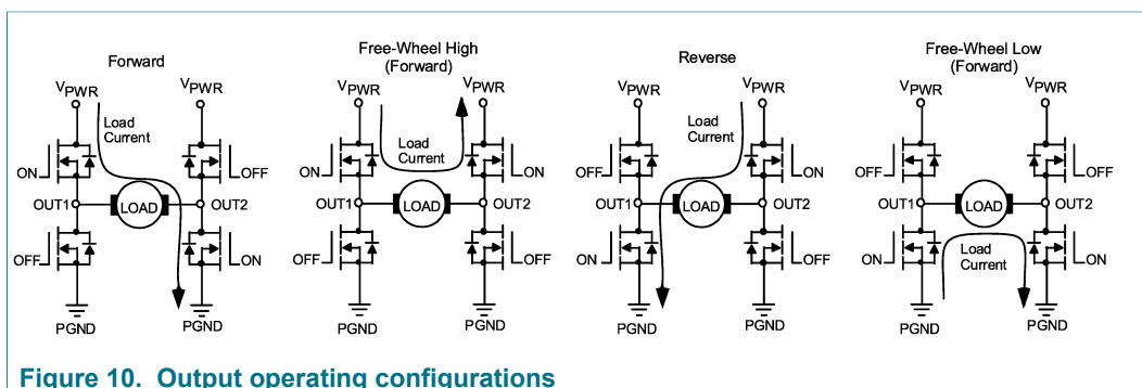
Figure 10. Output operating configurations
