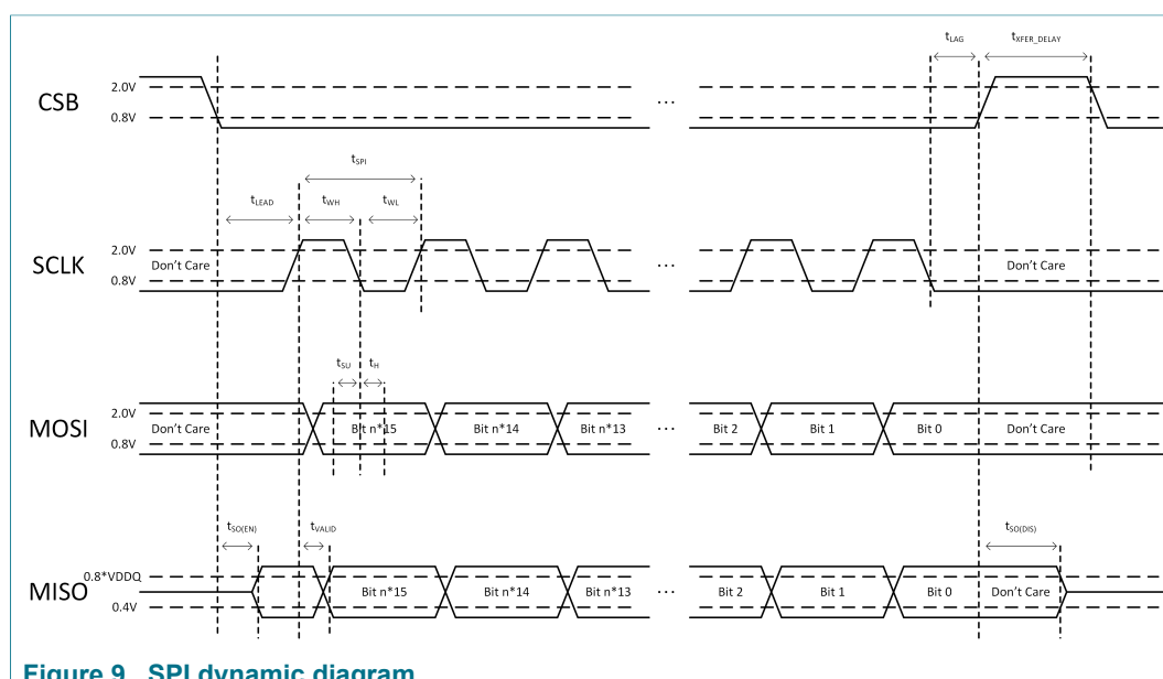
Figure 9. SPI dynamic diagram
