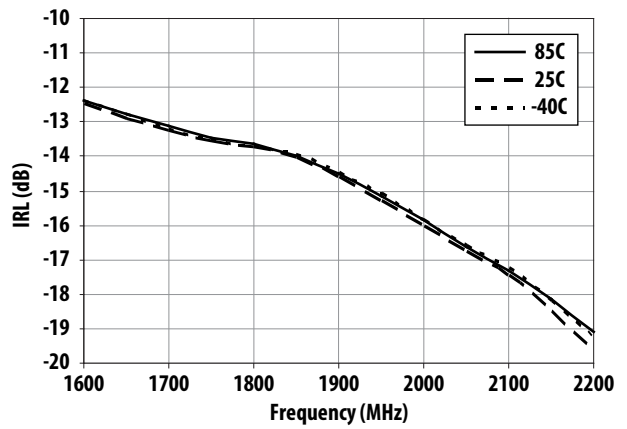
Figure 28. IRL vs Frequency and Temperature
