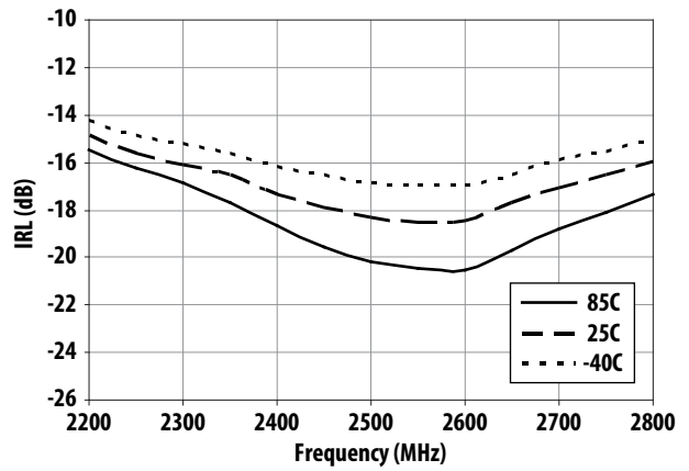
Figure 37. IRL vs Frequency and Temperature
