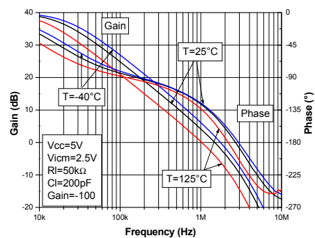
Figure 7. Voltage gain and phase with C_I = 200\text{ pF}
