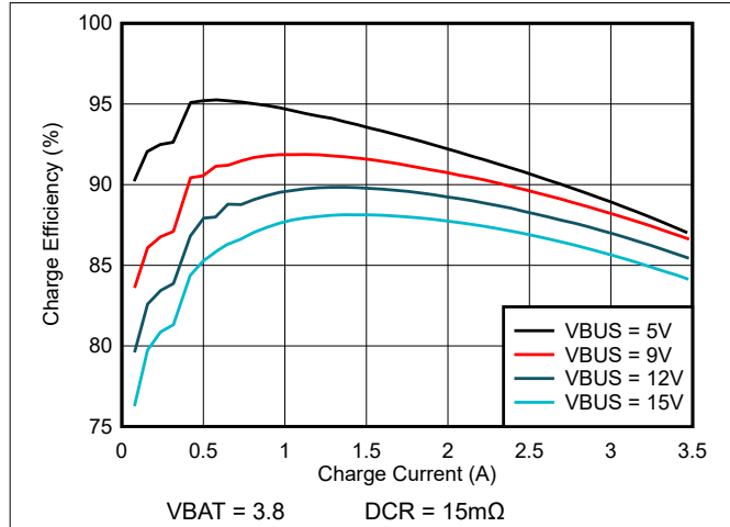
Figure 8-1. Charge Efficiency vs. Charge Current
