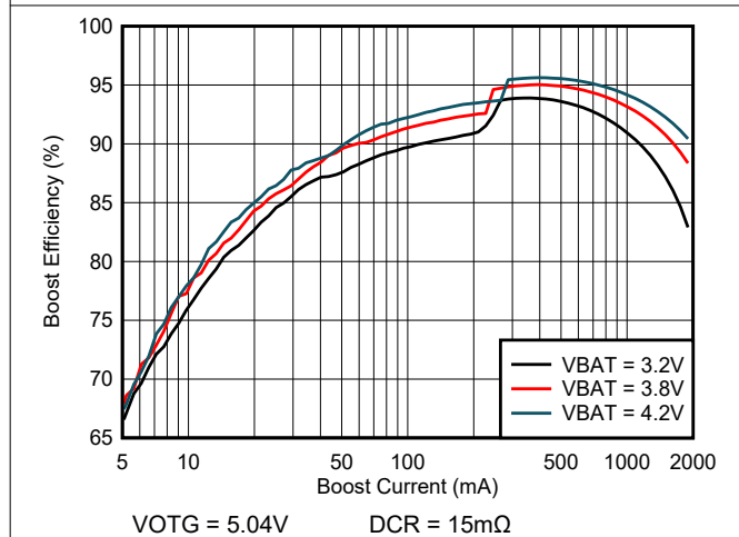
Figure 8-3. Boost Mode Efficiency vs. Boost Output Current
