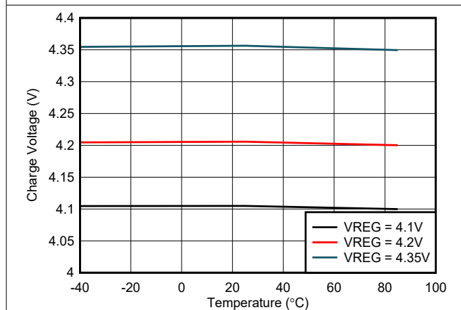
Figure 8-5. Charge Voltage Accuracy vs. VREG Setting
