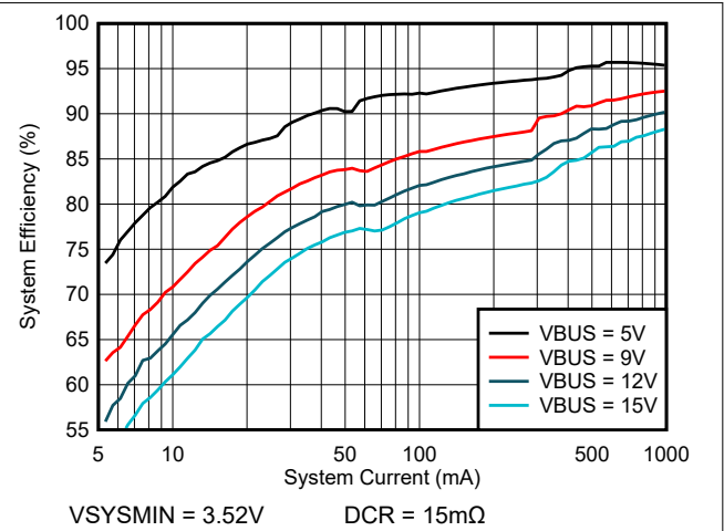
Figure 8-2. System Light Load Efficiency vs. System Current
