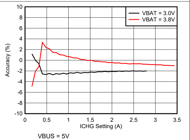
Figure 8-4. Charge Current Accuracy vs. ICHG Setting
