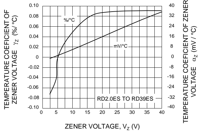
FIG.2 - TEMPERATURE COEFFICIENT vs. ZENER VOLTAGE
