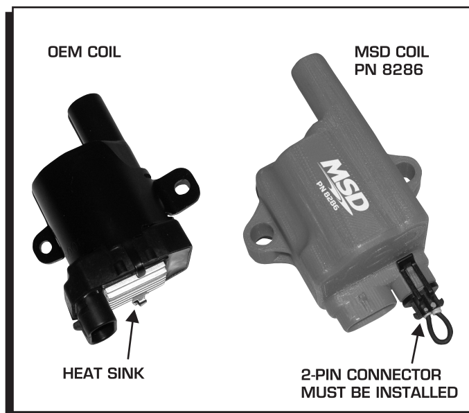
Figure 1 Coil Identification
