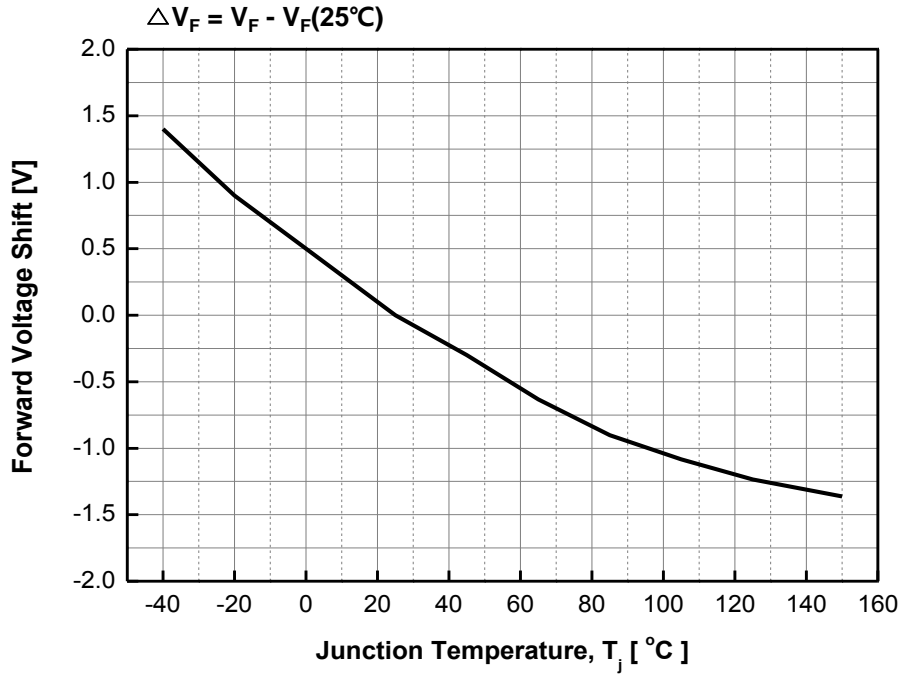
Fig 6. Junction Temperature vs. Forward Voltage Shift, I_F = 1.0A
