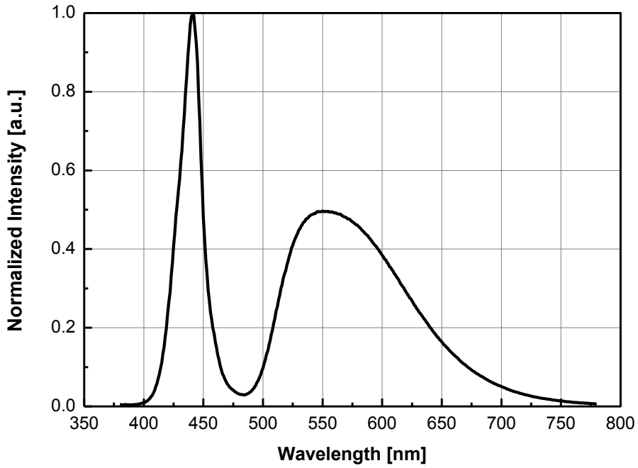
Fig 1. Color Spectrum, I_F = 1.0A , T_a = 25^\circ C
