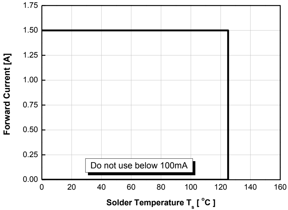
Fig 9. Solder Temperature vs. Allowable Forward Current.
