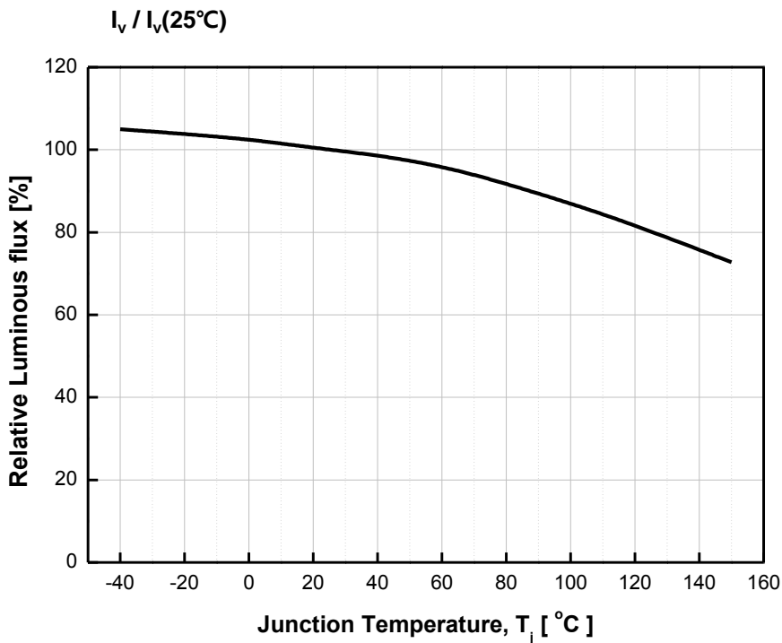
Fig 7. Junction Temperature vs. Relative Luminous Flux, I_F = 1.0A
