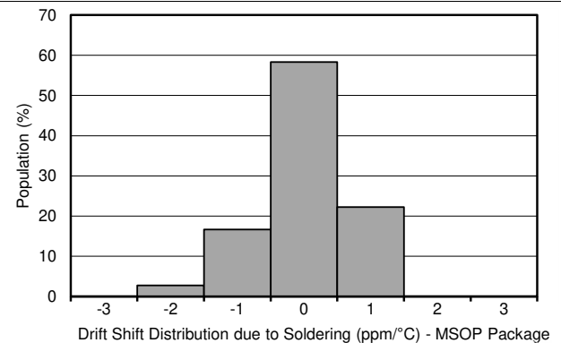
Figure 38. Drift Shift Distribution, VSSOP Package
